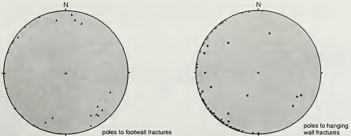
Figure 15 Equal-area lower hemisphere stereonet showing poles to fractures in Peoria Silt in the footwall and hanging wall of the English Hill fault at the Old Quarry trench.
